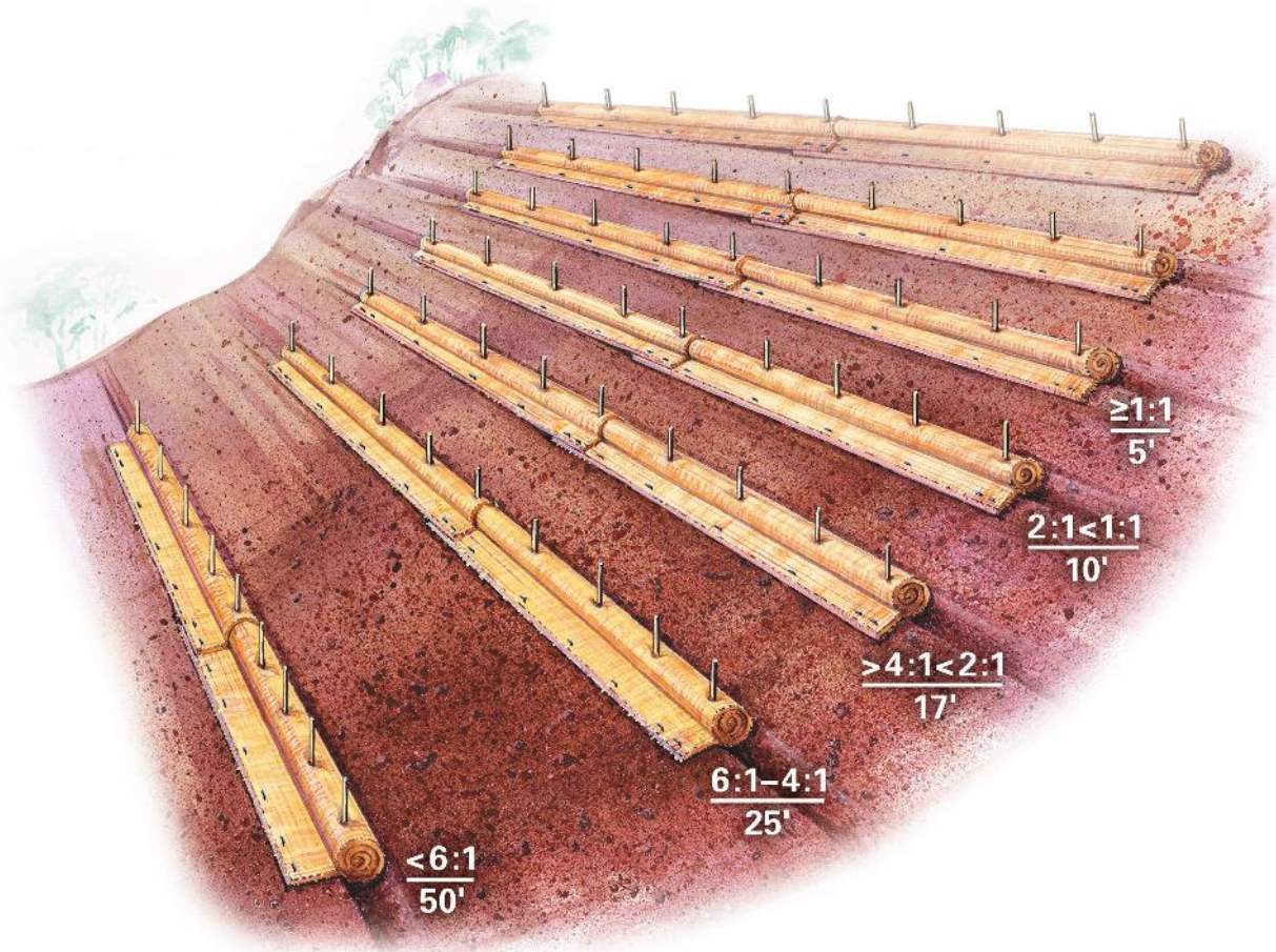
SediMax rolls should be installed along the slope contour with spacing based on slope grade.
